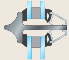
True Divided Lite Muntin Sightline: 7/8" exterior welded steel profile
