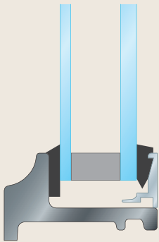
Fixed Frame Sightline: 1" Frame Depth: 1-3/4"
