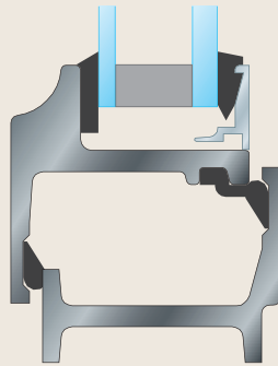
Operable/Door Frame Sightline: 2-3/16" Frame Depth: 2"
